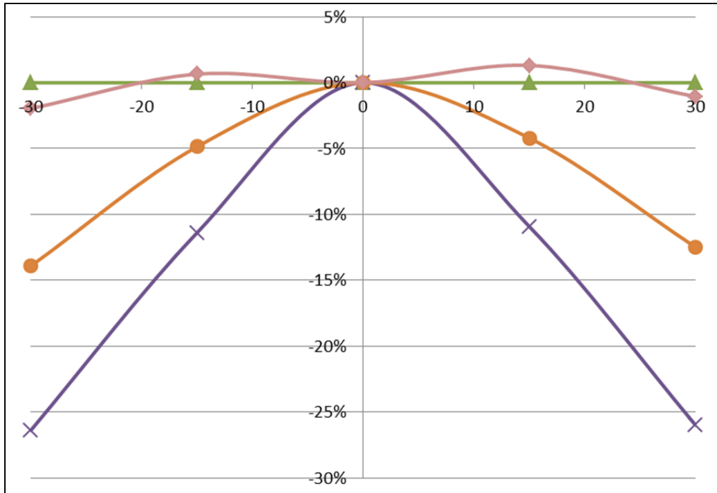
Figure 3. Sensitivity of the Beta Angle as a Function of Sign Twist
