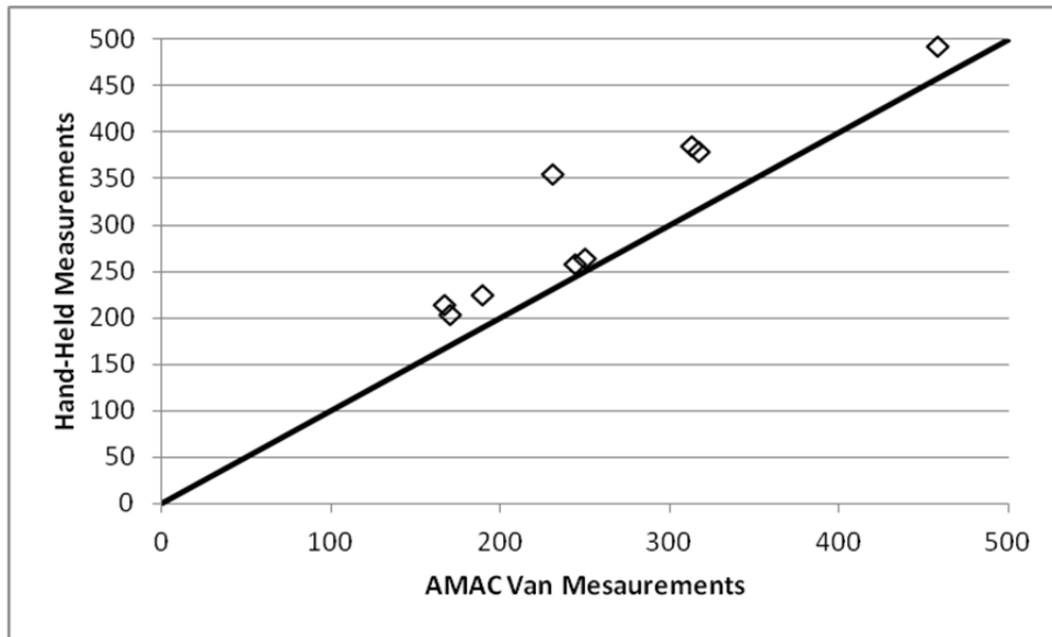
Figure 11. Comparison of Legend Measurements (cd/lx/m 2 )
