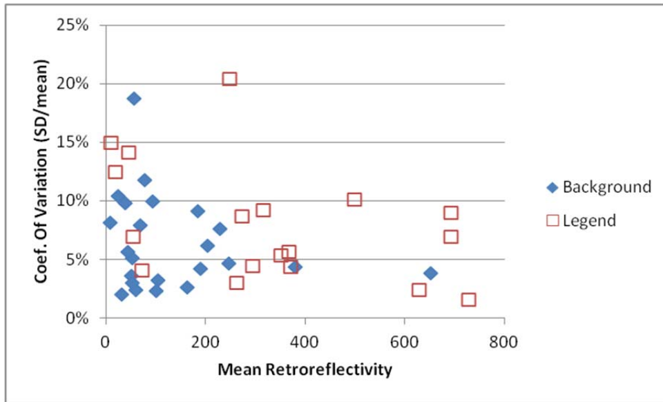
Figure 7. COV of Mobile Legend and Background Measurements
