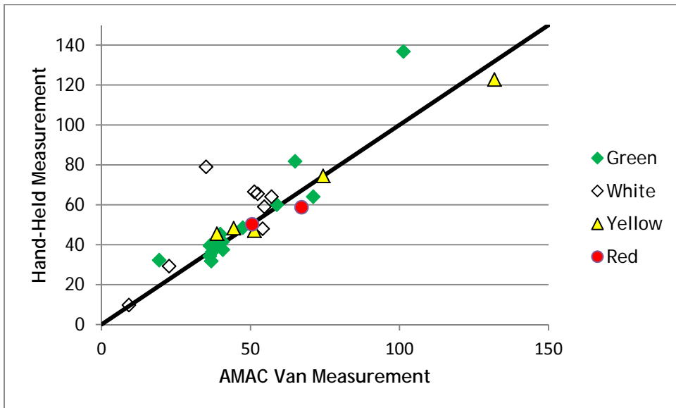
Figure 10. Close-Up of Comparison of Background Measurements ( \text{cd/lx/m}^2 )
