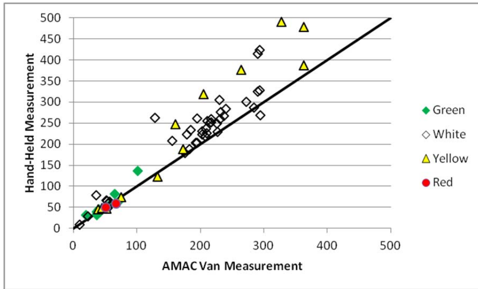
Figure 9. Comparison of Background Measurements ( \text{cd/lx/m}^2 )
