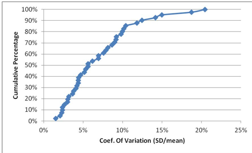
Figure 6. Cumulative Percentage of COV of Mobile Measurements
