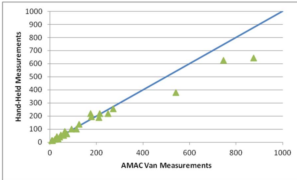
Figure 4. Comparison of Background Retroreflectivity Measurements (cd/lx/m 2 )
