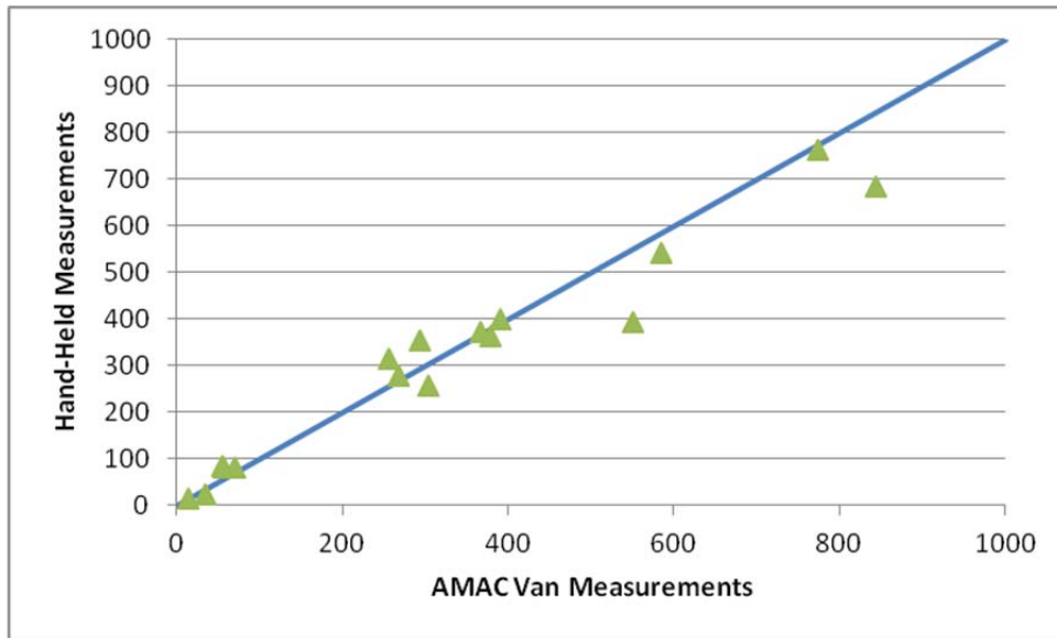
Figure 5. Comparison of Legend Retroreflectivity Measurements (cd/lx/m 2 )
