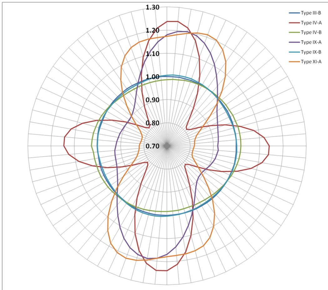
Figure 1. Rotational Sensitivity (Alpha=0.2°, Beta=4.0°)
